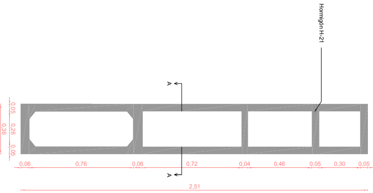
VISTA FRONTAL
